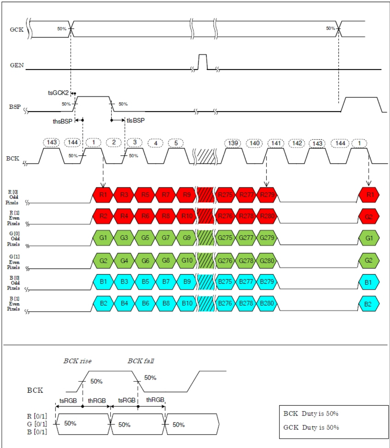
Figure: AC Timing 3
