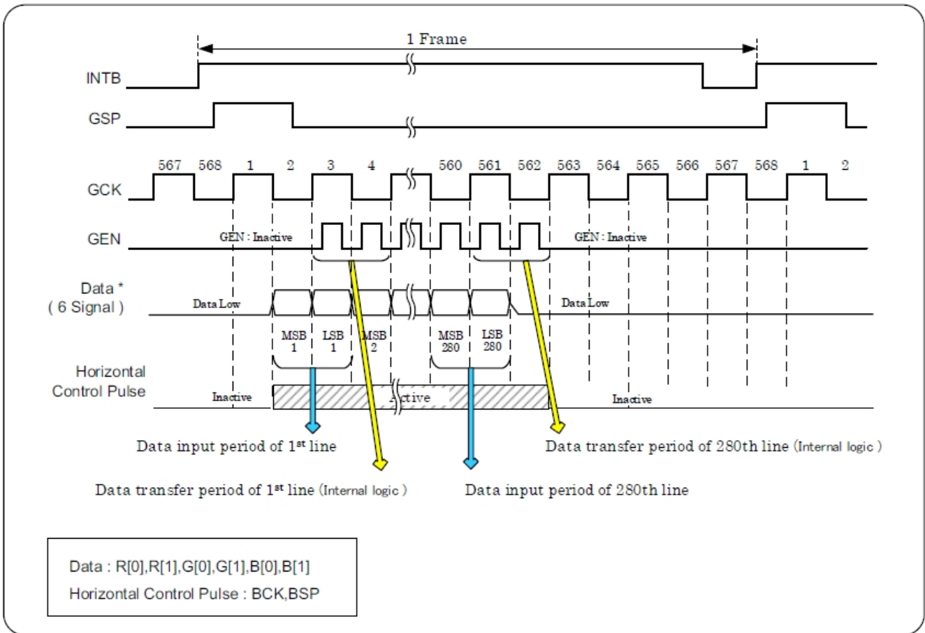
Figure: Vertical Diagram
