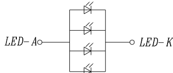
B/L Circuit
