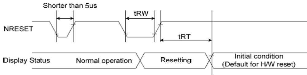
Figure 102 Reset Timing
