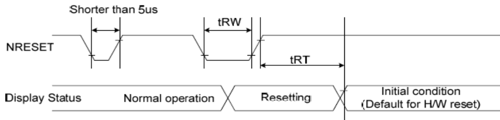
Figure 102 Reset Timing
