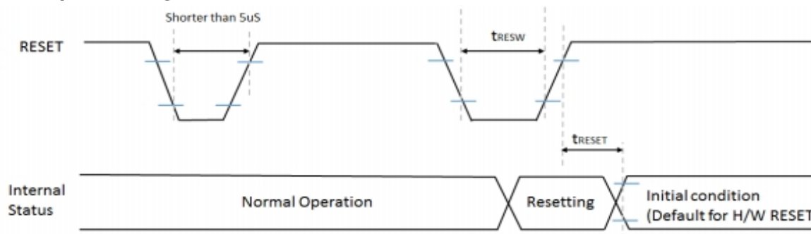
Figure 4-13 Reset Input Timing
