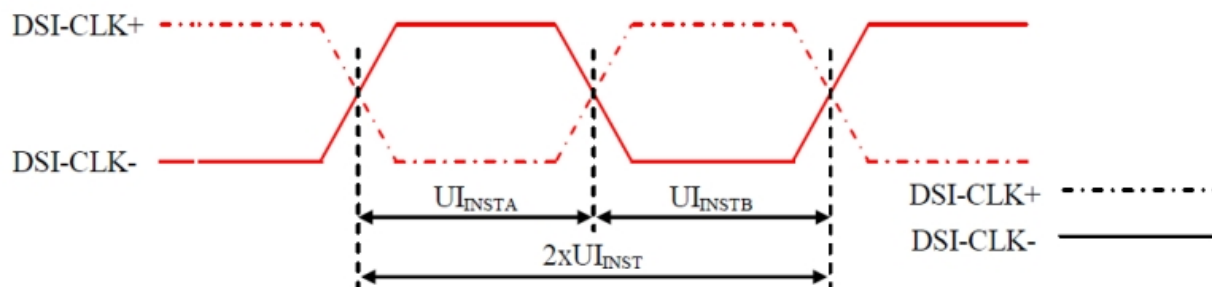
Figure 114 DSI Clock Channel Timing
