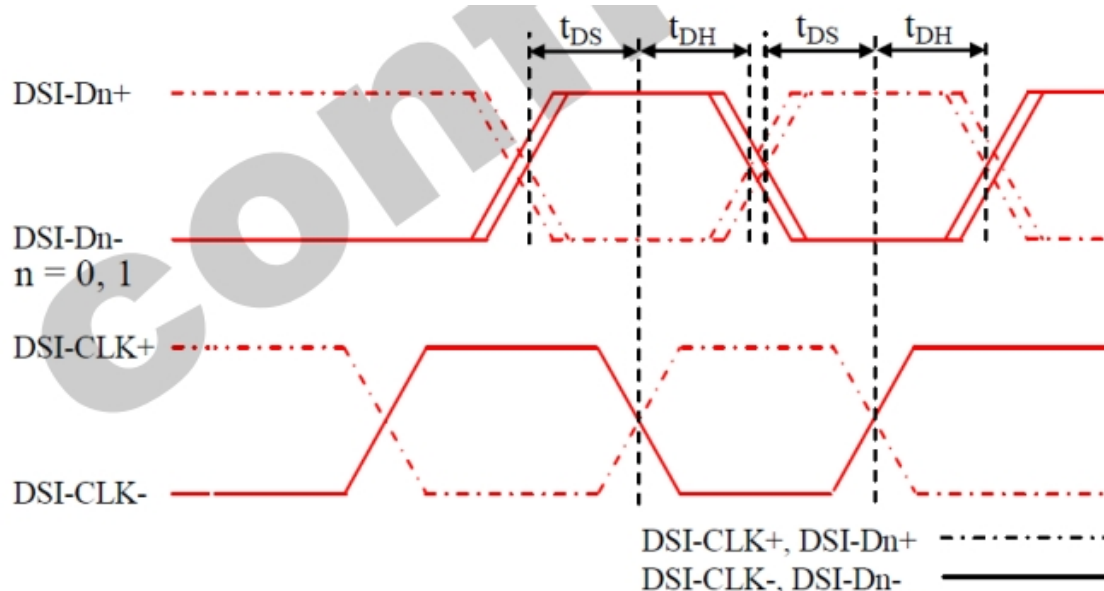
Figure 115 DSI Data to Clock Channel Timings
