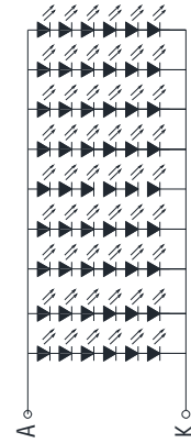
Backlight LED 6*9=54EA Circuit
