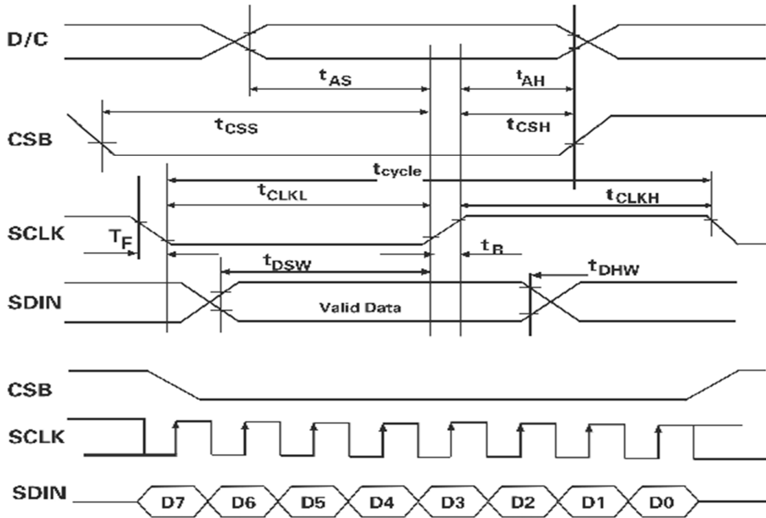
Figure 10-4-4: Serial interface characteristics
